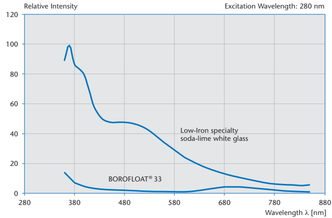
► Fluorescence Behavior of BOROFLOAT® 33 and Soda-Lime Glass Type for Different Wavelength Excitation
