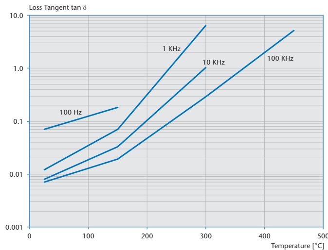
▶ BOROFLOAT® 33 – Loss Tangent as a Function of Temperature
