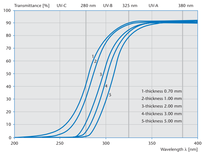
▶ BOROFLOAT® 33 – Transmittance in the UV Range
